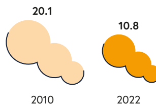
Population-weighted exposure to particulate matter in the six largest cities, in \mu\text{g}/\text{m}^3
