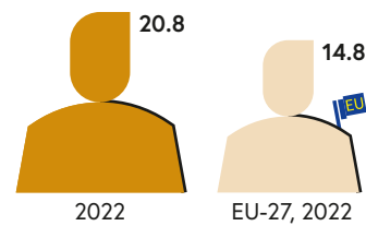
Recycling rate of waste excluding major mineral waste, in percent
