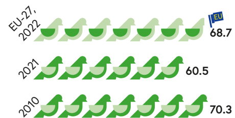
Farmland Bird Index (1998 = 100)
