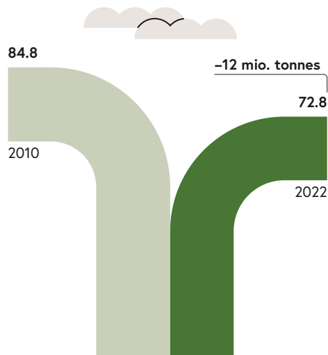
National greenhouse gas emissions, in million tonnes of CO 2 -equivalent
