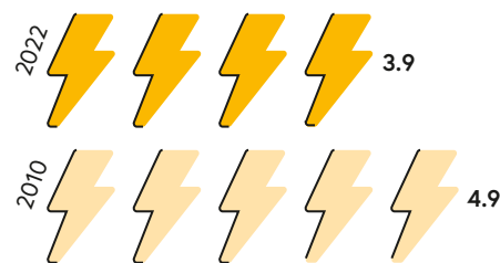
Energy intensity of gross domestic consumption, in megajoules
