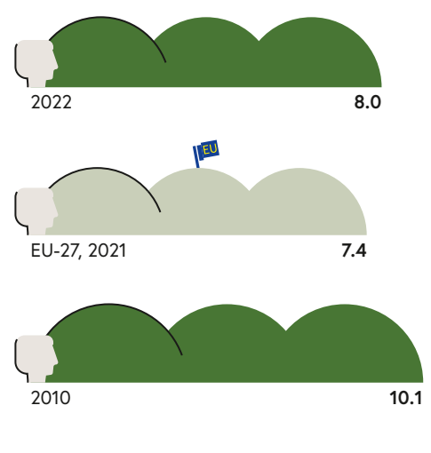
Greenhouse gas emissions per capita, in tonnes of CO 2 -equivalent
